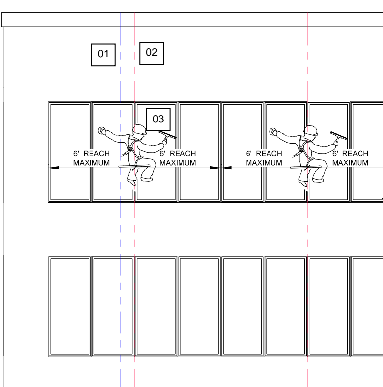
BUILDING ELEVATION
