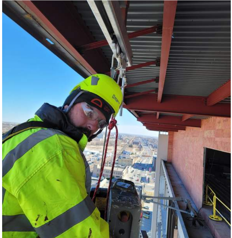
STANDING IN STAGE SUSPENDED FROM MONORAIL
